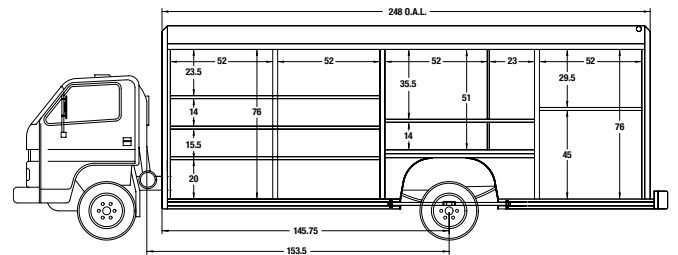
Chevrolet LCF Eight-Bay Conv. Capacity: 405 batteries* Access: side load GVW: 29,000 - 33,000 Bays: 52", 52", 77.5", 52"
