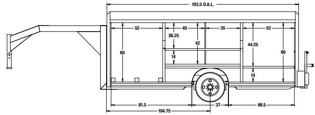
Gooseneck Trailer Capacity: 180 batteries* Access: side load GVW: 12,699 Bays: 52", 40", 35", 52"
