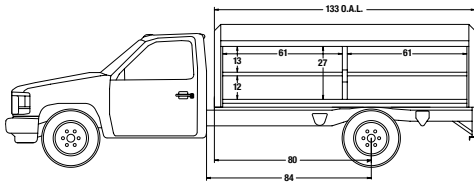
Four-Bay Mini for GMC/Chevrolet HD3500 Capacity: 127 batteries* Access: side load GVW: 13,400 Bays: 61"
