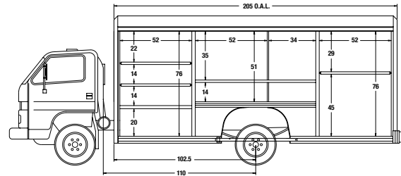
Chevrolet LCF Six-Bay Conv. Capacity: 275 batteries* Access: side load GVW: 25,900 - 28,000 Bays: 52", 52", 34" plus bay, 52"
