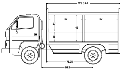
Chevrolet LCF Four-Bay Mini Cab-over Capacity: 160 batteries* Access: side load GVW: 13,500 - 15,500 Bays: 57"
