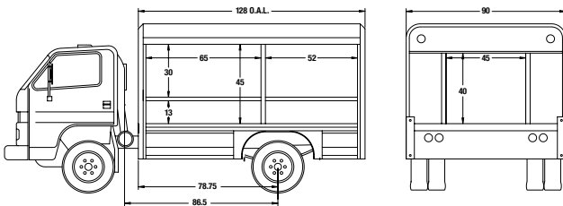
Chevrolet LCF Four-Bay Mini Rear Loader (also available in cab-over version) Capacity: 164 batteries* Access: rear and side load GVW: 15,000 - 21,000 Bays: 65", 52", 45" rear bay
